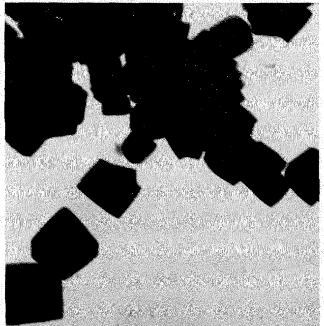
FIG. 3—Cubic particles of magnesium oxide enlarged 20,000 diameters.
